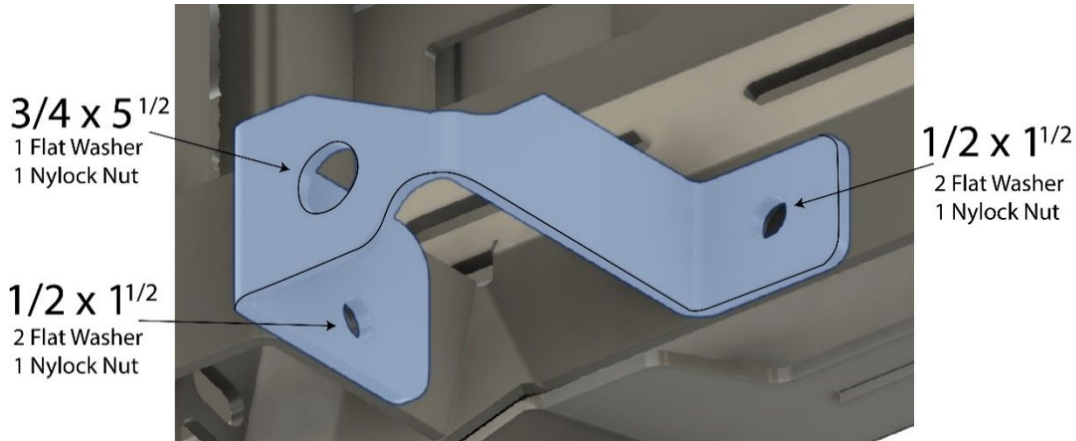
Figure 7: Differential bracket
