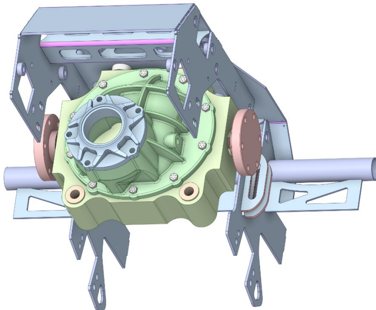
Figure 5: Two models of rear differential install
