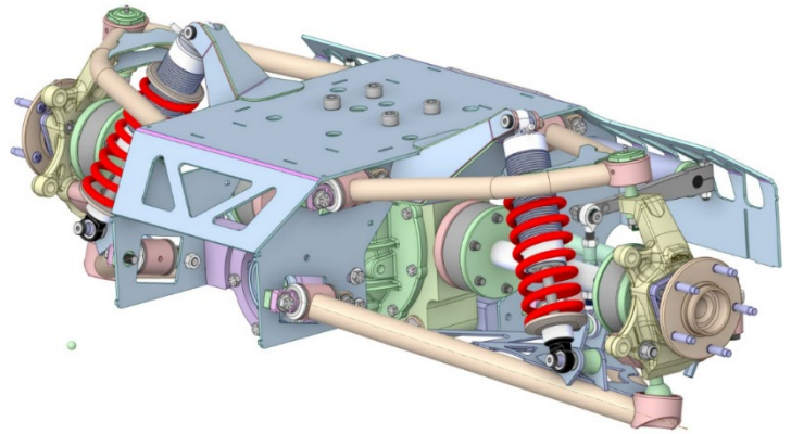
Figure 13: Traditional mount shock install
