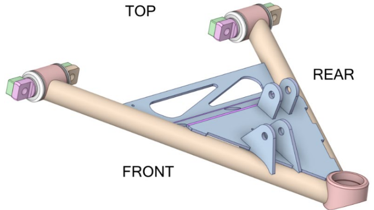
Figure 8: A model and close up of the lower control arms
