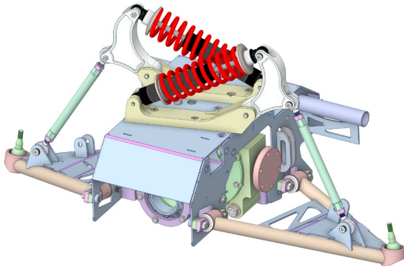
Figure 15: Adding the push rod onto the assembly
