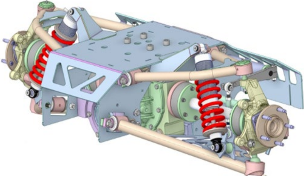
Figure 4: One model of traditional shock mount overview
