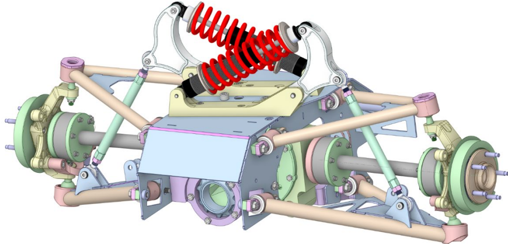
Figure 17: Upper control arm installment
