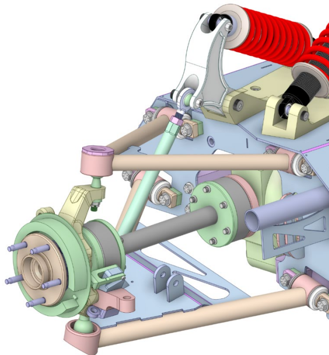
Figure 18: CV axle installment
